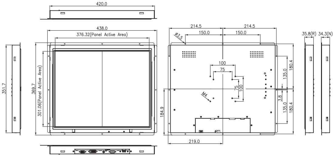
Figure 2.1 IDS-3119 Series Dimensions
