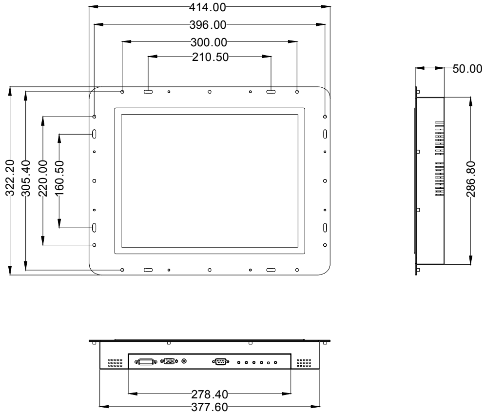
Figure 3-1: Dimensions of the ES-3115G/R/C/S/V-XA
