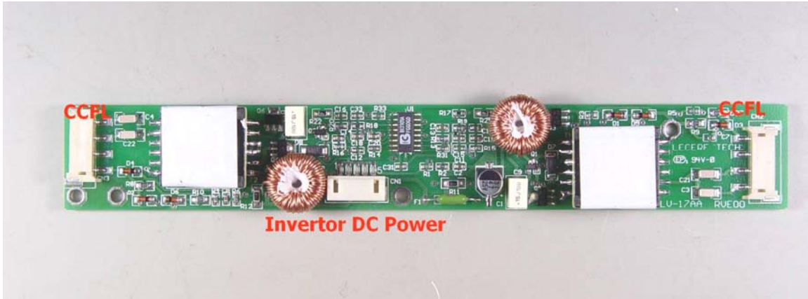
Figure 3-10: Locating connectors on DC/AC inverter
