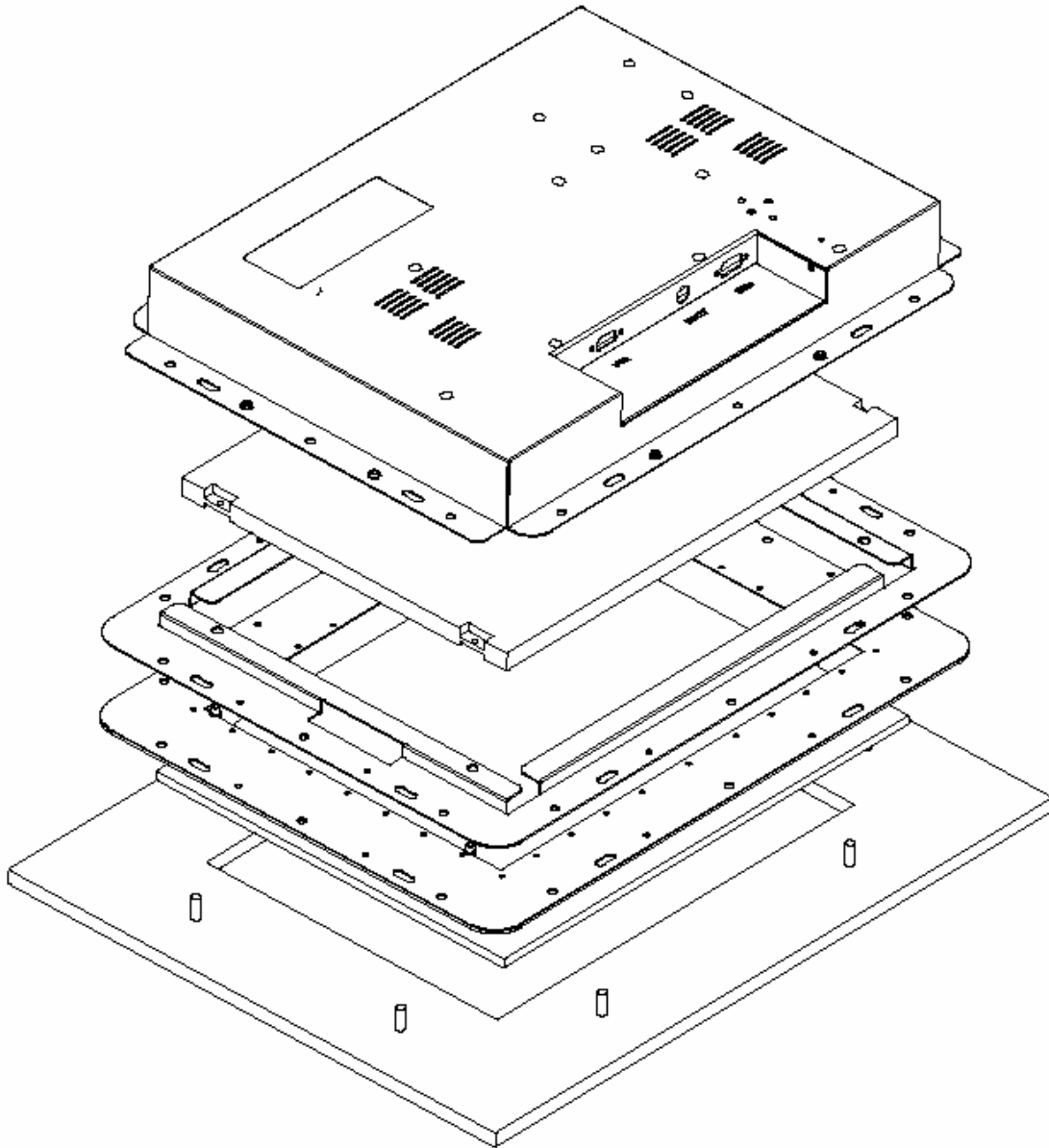
Figure 3-7: Exploded diagram of the ES-3115S/ V –XA
