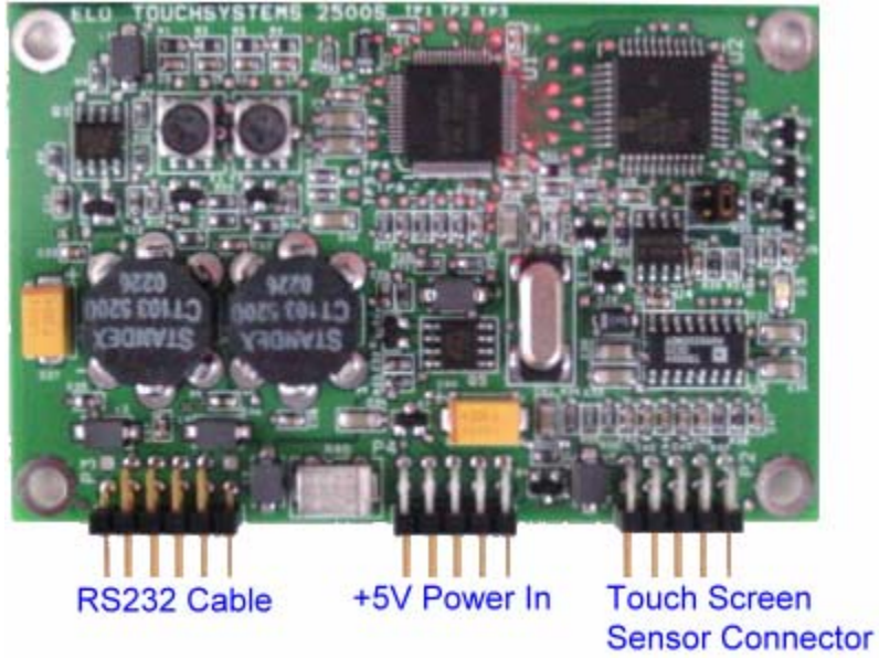
Figure 3-13: Locating connector of ES-3115S and ES-3115V control board
