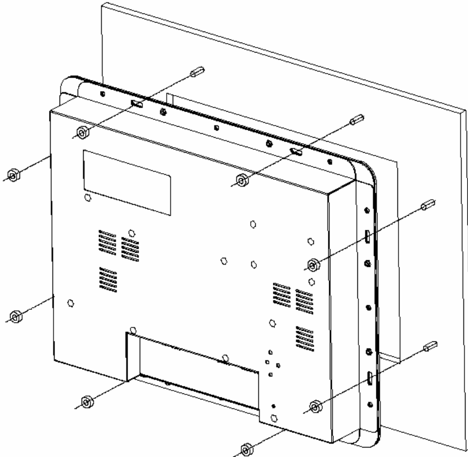
Figure 3-4: Rear mounting of the ES-3115 G/R/C/S/V-XA
