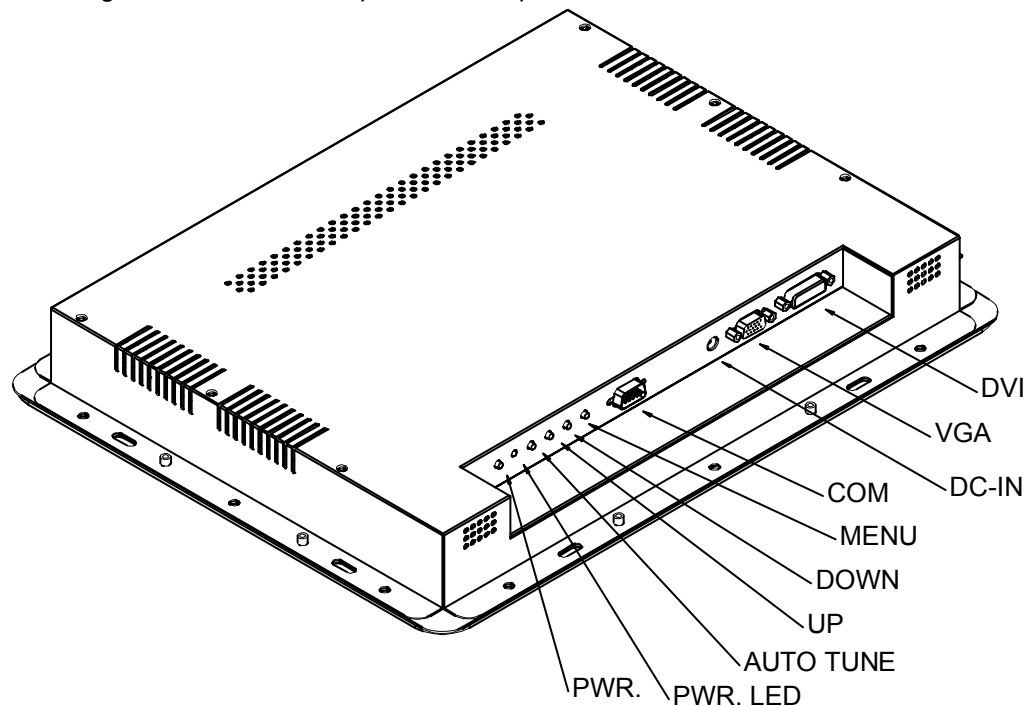
Figure 2-1: Rear view of the ES-3115R/C/S/V
