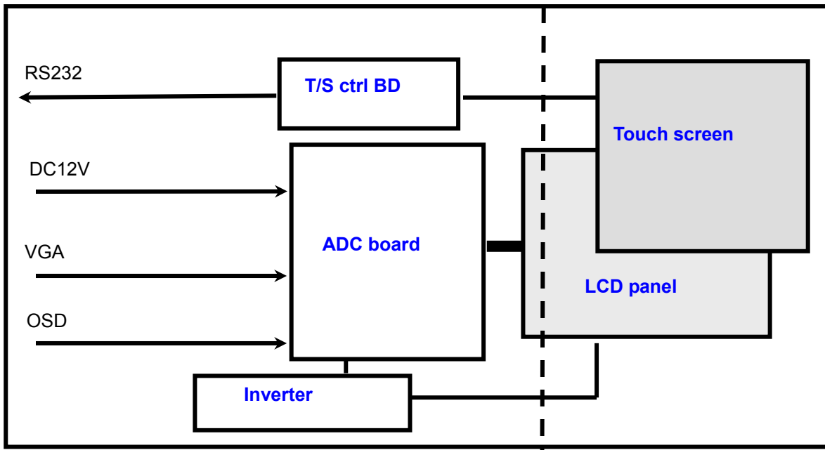
Figure 3-8: Block Diagram
