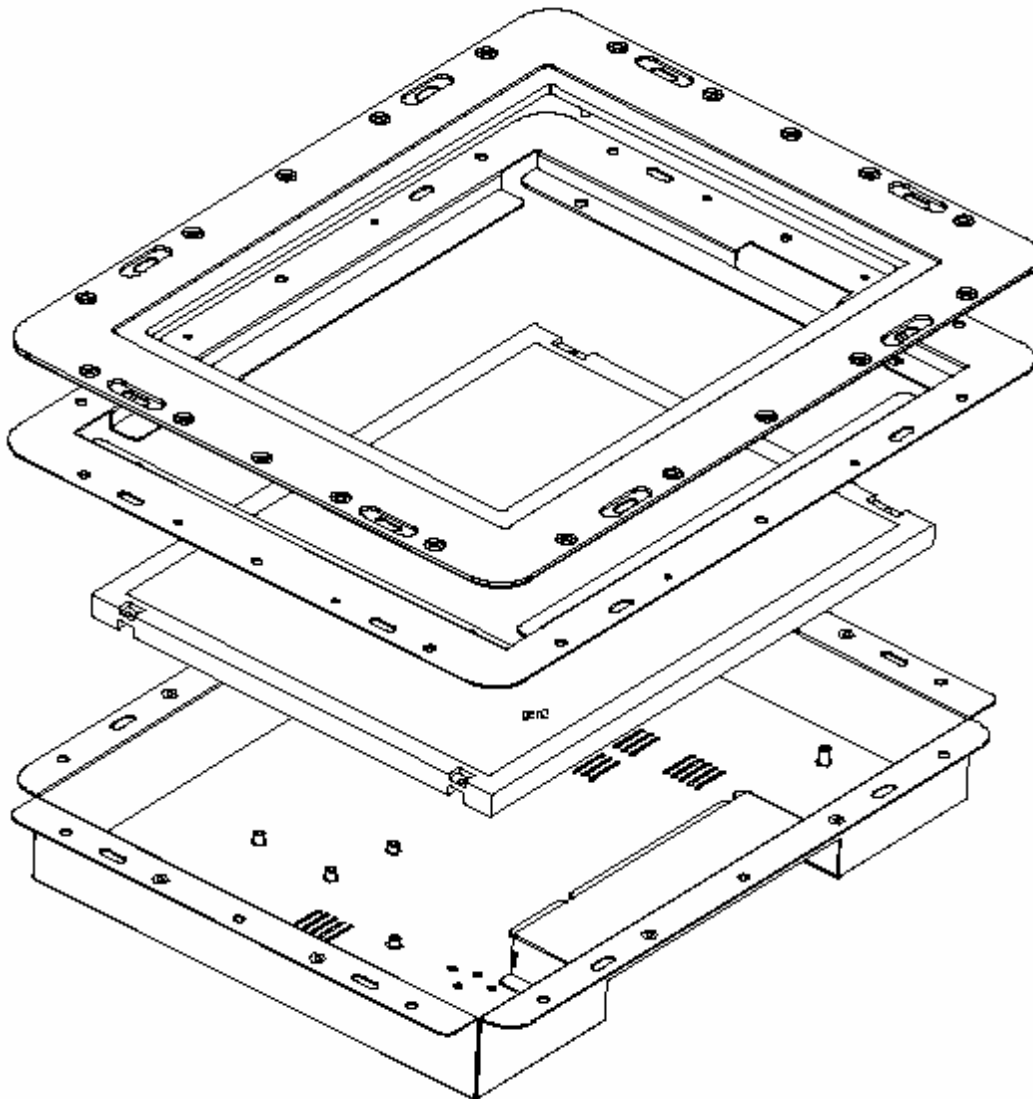
Figure 3-6: Exploded diagram of the ES-3115 G/R/C-XA
