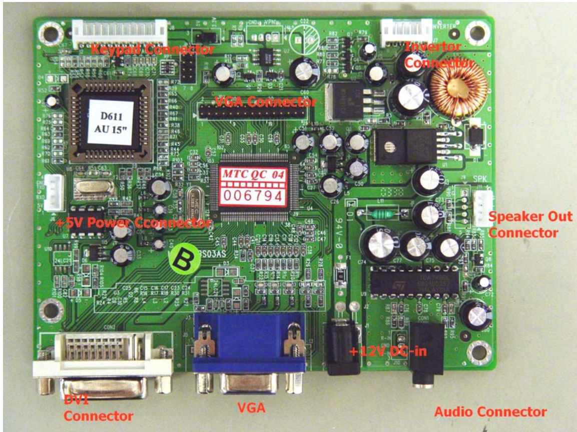
Figure 3-9: Locating connectors on ADC board
