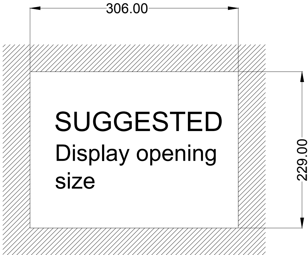
Figure 3-3: ES-3115 G/R/C/S/V-XA dimensions of cut-off.
