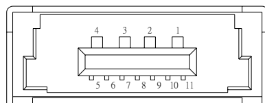
Figure 2.7 eSATA/USB Connector
