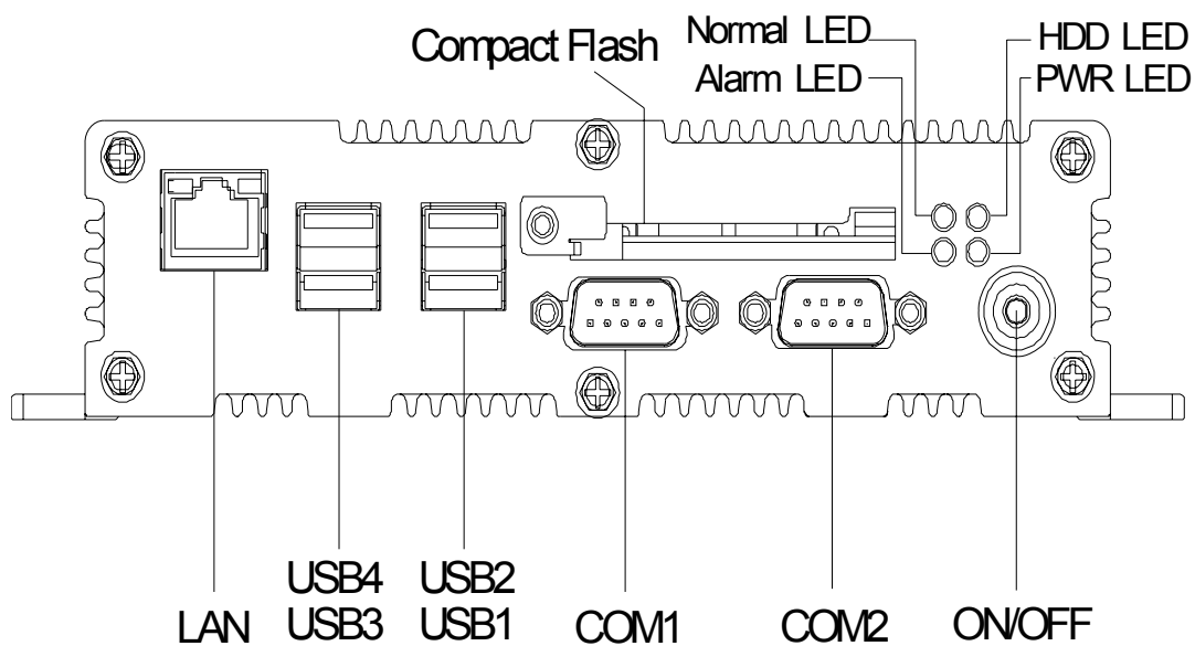
Figure 2.1 ARK-1382 Front Side External I/O Connectors
