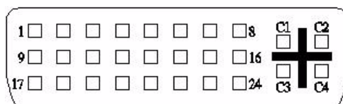
Figure 2.6 DVI-I Connector
