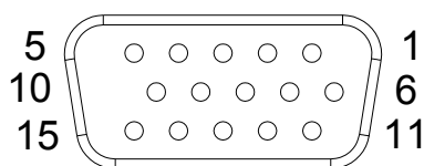
Figure 2.18 VGA Connector
