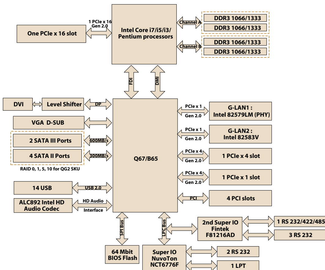
Figure 1.3 AIMB-781 Block Diagram
